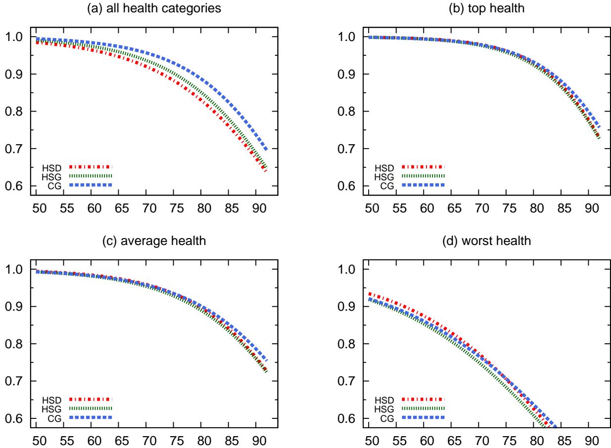
Figure 6: Survival rates
