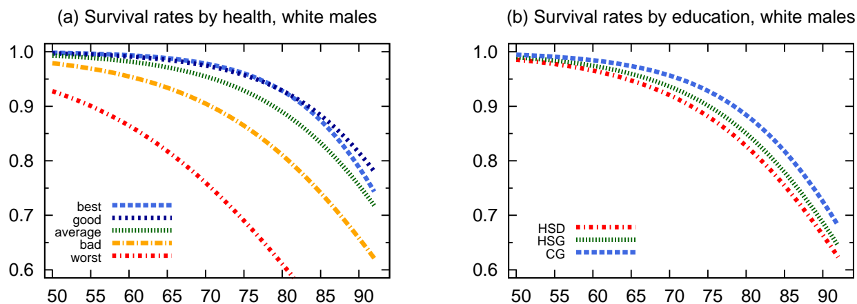
Figure 5: Survival rates
